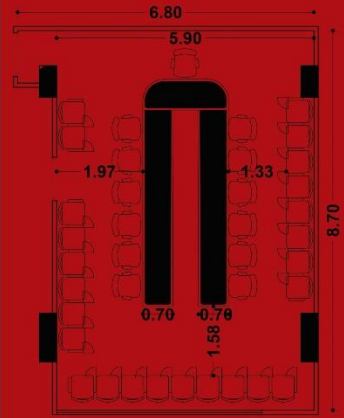
LAYOUT PLAN
