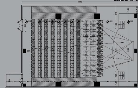
LAYOUT PLAN
